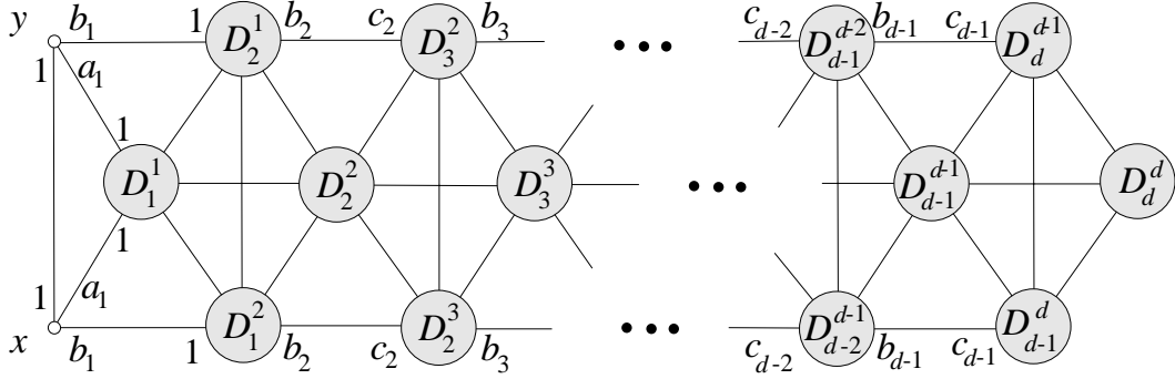
Figure 2.1: Distance distribution corresponding to an edge. Observe: D_{i-1}^{i-1} \cup D_i^i \cup D_{i+1}^{i+1} = \Gamma_i(x) for i = 1, \dots, d . The number beside edges connecting cells D_i^j indicate how many neighbours a vertex from the closer cell has in the other cell, see Lemma 2.11.
