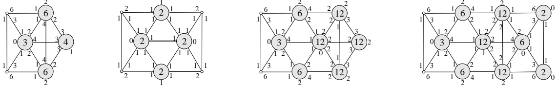
Figure 4.1: The 1-homogeneous partition for the complement of the triangular graph T(7) , the icosahedron, the Doro graph and the Conway-Smith graph.
