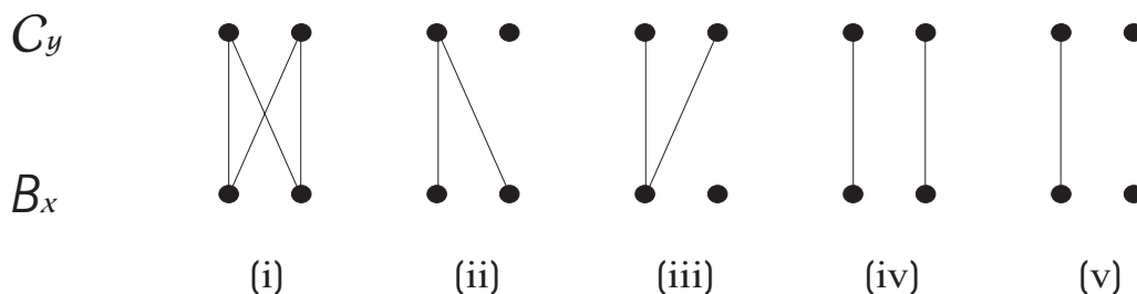
Figure 2: Bipartite graphs induced by pairs of blocks
