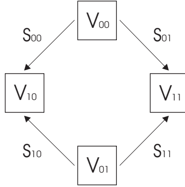
Figure 1: Bipartite tetracirculant \mathcal{F}(S_{00}, S_{01}, S_{10}, S_{11})
