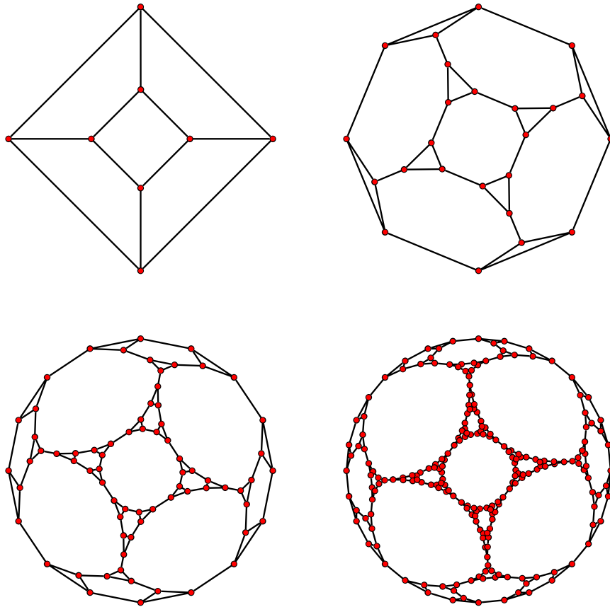
Figure 2: Cube and its first 3 repeated truncations.
