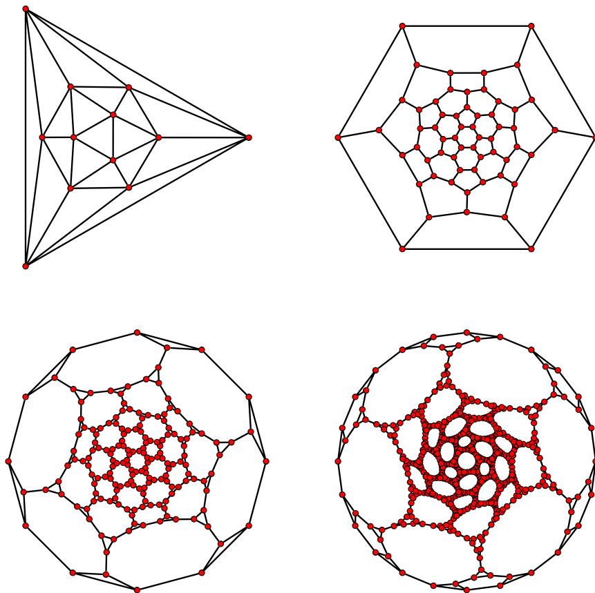
Figure 3: Icosahedron and its first 3 repeated truncations.
