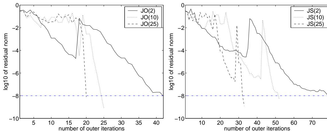
FIG. 7.2. Convergence plot for the exterior eigenvalue (\lambda_{\max}, \mu_{\max}) for n = 100 and u = v = [1 \ \dots \ 1]^T . The plots show the \log_{10} of the residual norm \rho_k (3.3) versus the outer iteration number k for the Jacobi–Davidson type method for the eigenvalue (\lambda_{\max}, \mu_{\max}) using 2 (solid line), 10 (dotted line), and 25 (dashed line) GMRES steps to solve the correction equation with orthogonal projections (left plot) and skew projections (right plot), respectively.
