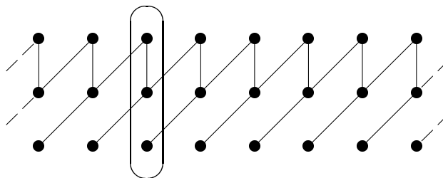
Figure 1: Rotagraph and its fiber
