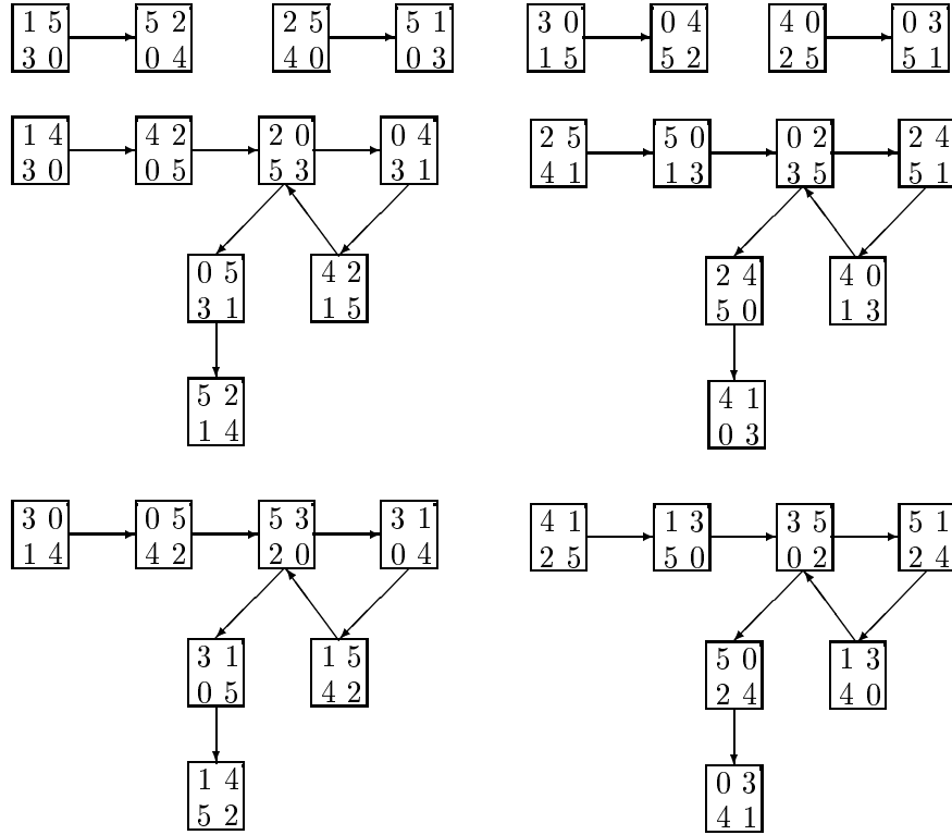
Figure 2: Graph D_2(P_2; X) (without isolated vertices)
