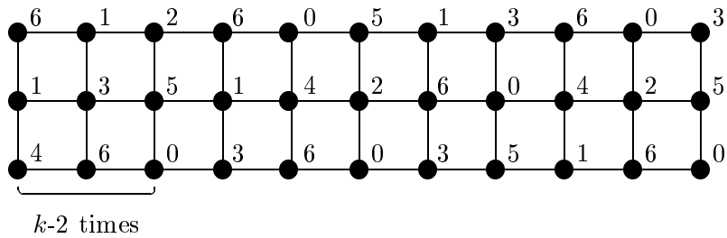
Figure 5: 6- L(2, 1) -coloring of C_{3k+2} \square P_3 , k \geq 2
