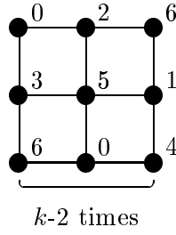
Figure 3: 6- L(2, 1) -coloring of C_{3k} \square P_3 , k \geq 1
