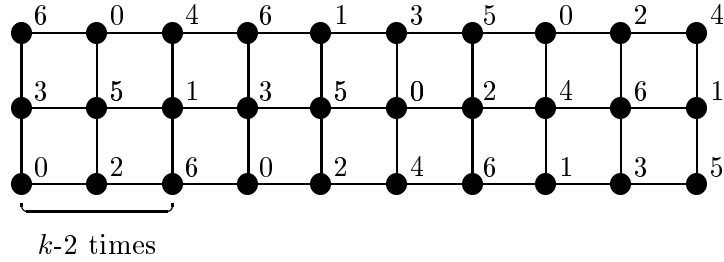
Figure 4: 6- L(2, 1) -coloring of C_{3k+1} \square P_3 , k \geq 2
