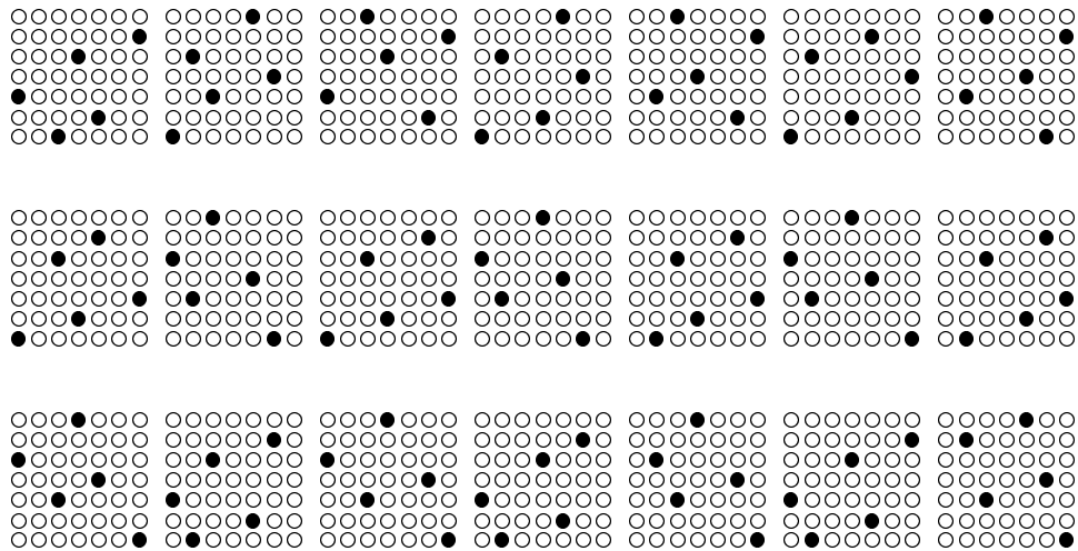
Figure 6: 105 independent vertices of C_7 \boxtimes C_7 \boxtimes C_{21}
