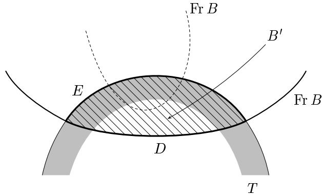
Figure 4: Inner disk D with respect to T
