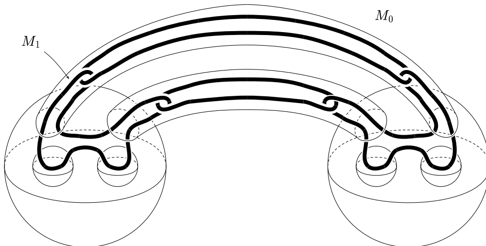
Figure 6: Example of g(X \cup Y) = g(X) + g(Y) + 1
