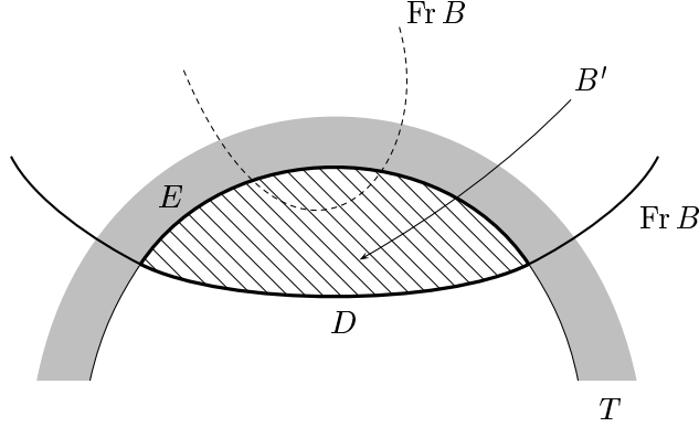
Figure 5: Outer disk D with respect to T
