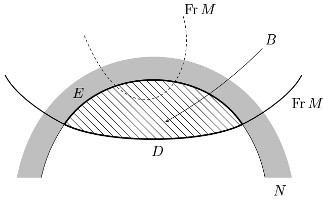
Figure 2: Inner disk D with respect to N
