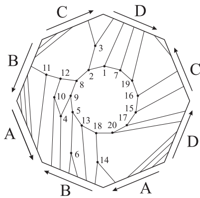
Figure 19: S_n6 embedded into double torus.
