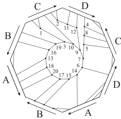
Figure 18: S_n5 embedded into double torus.
