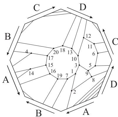
Figure 20: S_n7 embedded into double torus.
