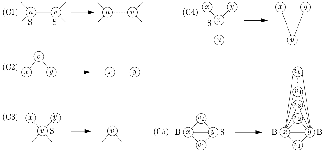
Figure 1: Forbidden configurations and their reductions.
