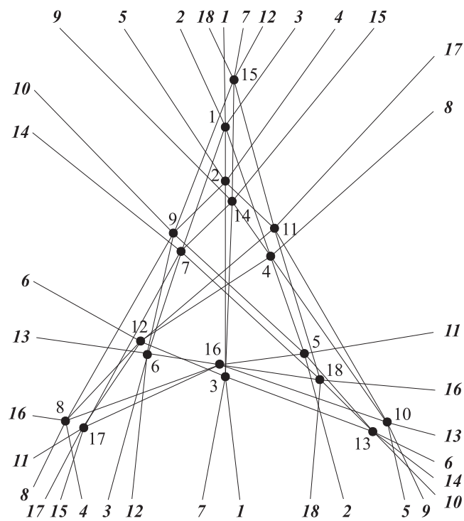
Figure 9: A schematic diagram (pseudoline configuration) of the triangle-free 18-B configuration as a “double cover” of the Pappus configuration.
