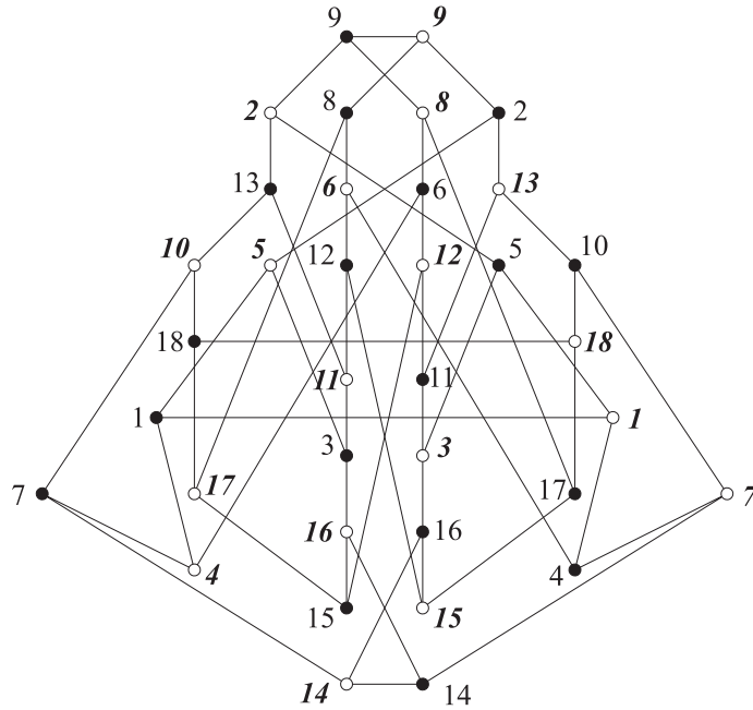
Figure 5: The Levi graph of the configuration 18-A.
