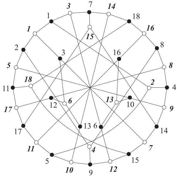
Figure 7: The Levi graph of the configurations 18-B (plain font) and 18-C (italic)
