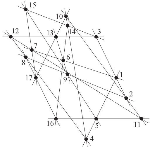
Figure 4: A geometric realization of the triangle-free configuration (17_3) .
