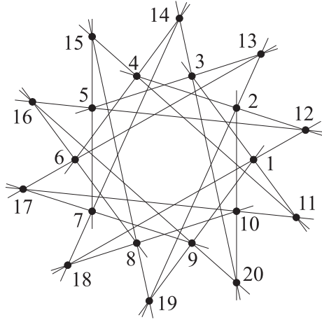
Figure 14: A geometrically selfpolar astral realization of the flag transitive triangle-free configuration (20_3) .
