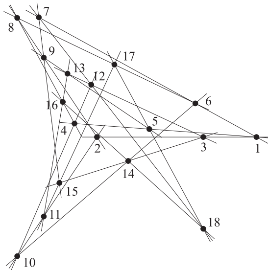
Figure 10: A geometric realization of the 18-C configuration.
