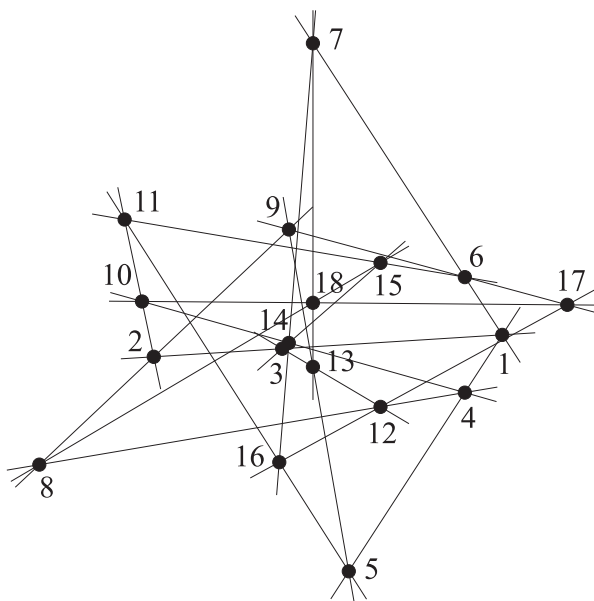
Figure 6: A geometric realization of the 18-A configuration.
