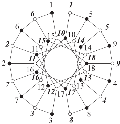
Figure 11: The Levi graph of the triangle-free combinatorially selfpolar configuration 18-D. This graph is the generalized Petersen graph G(18, 5) .
