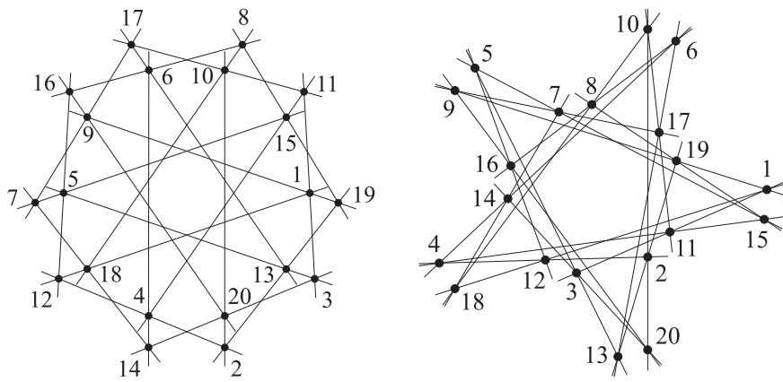
Figure 15: Two dihedral astral realizations of the flag transitive triangle-free configuration (20_3) .
