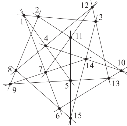
Figure 2: A stellar realization of the Cremona-Richmond (15_3) configuration.
