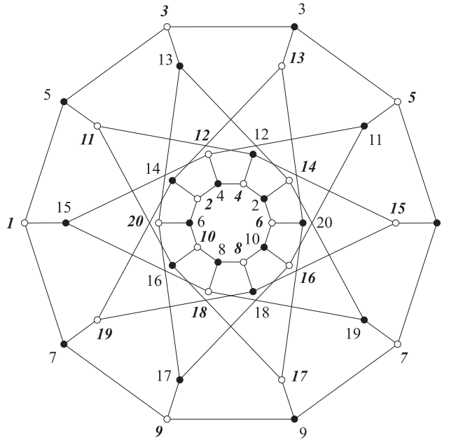
Figure 13: The Levi graph of the flag transitive triangle-free cconfiguration (20_3) . It is the Kronecker double cover of the dodecahedron graph G(10, 2) .
