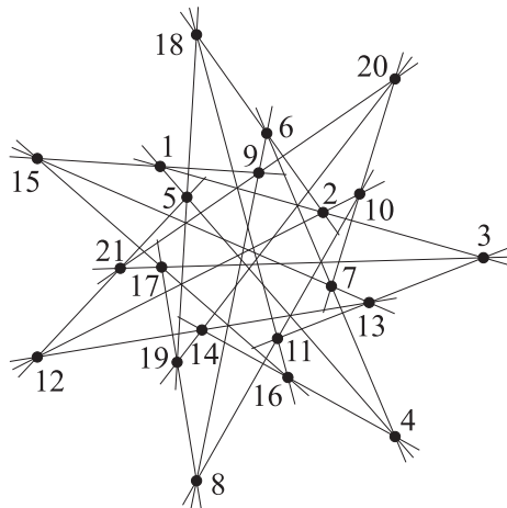
Figure 17: A stellar realization of the unique point transitive triangle-free configuration (21_3) .
