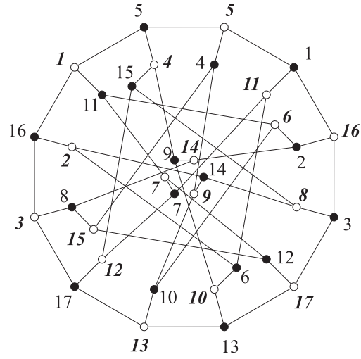
Figure 3: Levi graph of the triangle-free combinatorially selfpolar configuration (17_3) .
