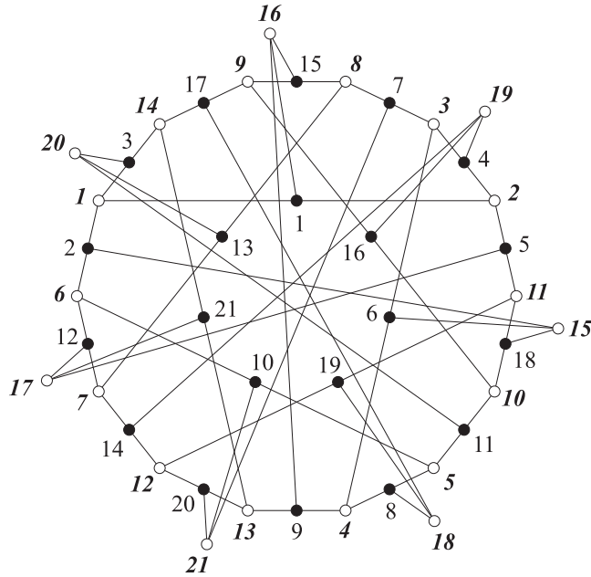
Figure 16: The Levi graph of the unique point transitive triangle-free configuration (21_3) . The picture above is from [1] and was obtained by subdividing the Heawood graph (Levi graph of the Fano configuration) and connecting each set of 3 “collinear” vertices with valency 2 to a new vertex. The vertices of the Heawood graph correspond to the lines of the larger line orbit, the subdivision points correspond to the points, while the “new vertices” correspond to the lines of the smaller line orbit.
