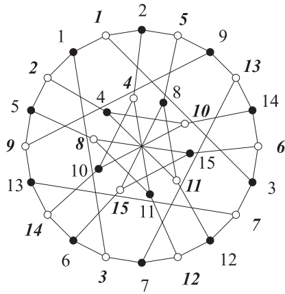
Figure 1: The Levi graph of the triangle-free combinatorially selfpolar Cremona-Richmond (15_3) configuration. This graph is the Tutte 8-cage.
