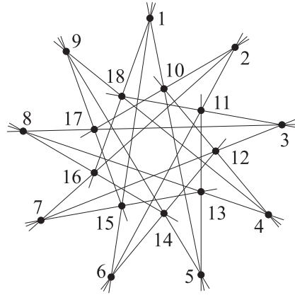
Figure 12: A geometrically selfpolar astral realization of the triangle-free configuration 18-D.
