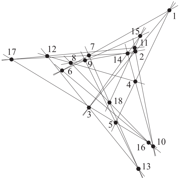
Figure 8: A geometric realization of the 18-B configuration.
