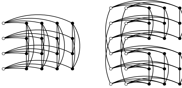
Figure 1: The graphs \Gamma_{1,4} and \Gamma_{2,3} . Green vertices are depicted by empty circles and red vertices by full ones.
