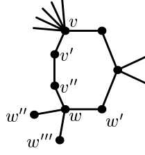
Figure 1: Notation used in the proof of Lemma 8.
