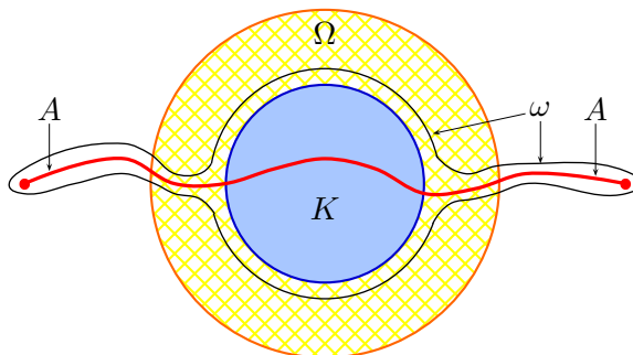
FIGURE 1. Theorem 2.1
