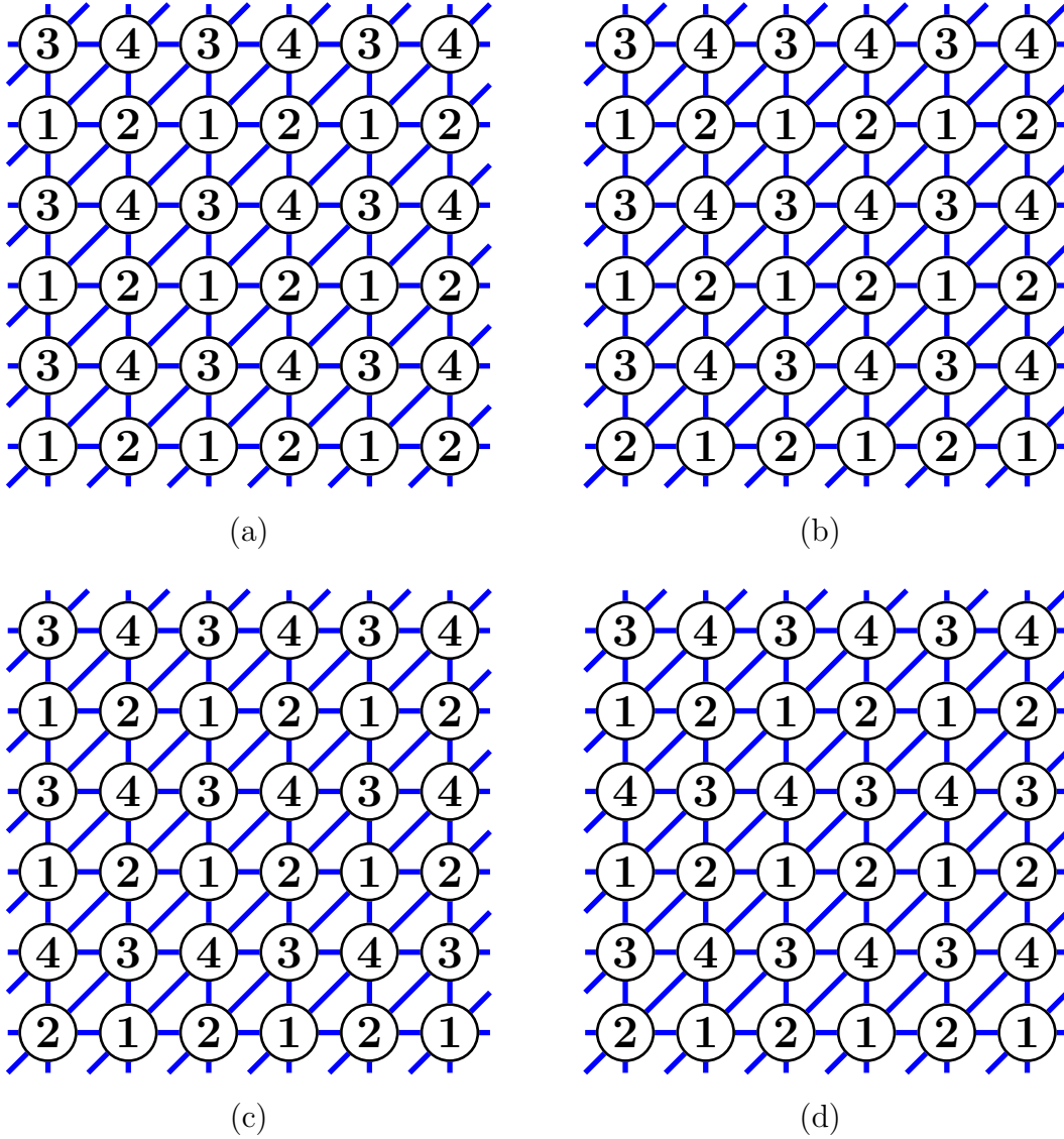
Figure 4: Four-colorings of the triangulation T(6, 6) . (a) Coloring c_{ns} (3.1) with |\deg(c_{ns})| = 18 . (b) Coloring f_b obtained from c_{ns} by swapping colors 1, 2 on the bottom row. (c) Coloring f_c obtained from f_b by swapping colors 3, 4 on the second row from the bottom. (d) Coloring f_d obtained from f_b by swapping colors 3, 4 on the fourth row from the bottom. The coloring c_{ns} in (a) has |\deg(c_{ns})| = 18 ; the colorings f_i in (b)–(d) have |\deg(f_i)| = 6 .
