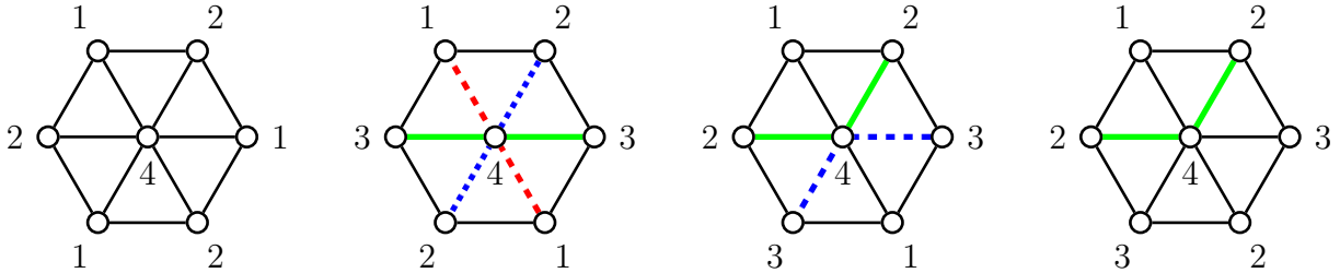
Figure 2: Non-singular edges around a vertex.
