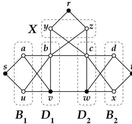
FIGURE 7. Labeled graph G
