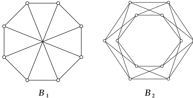
FIGURE 2. Two graphs that are not BG-graphs
