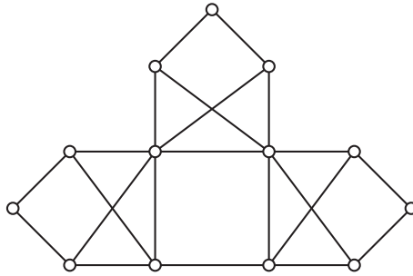
FIGURE 6. The graph G
