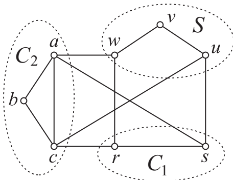
FIGURE 3. Graph G for one-half argument example
