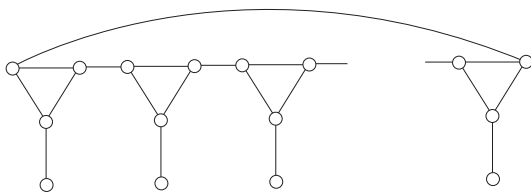
FIGURE 5. A claw-free graph with \alpha(G) = 2\gamma(G)
