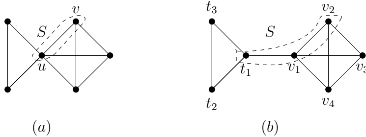
Figure 1: The configurations of Claims 11 and 12.
