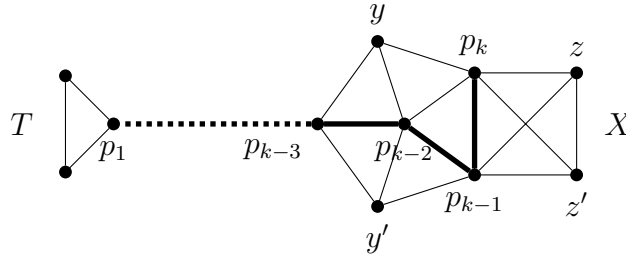
Figure 3: Positions of T , X , y and y' .
