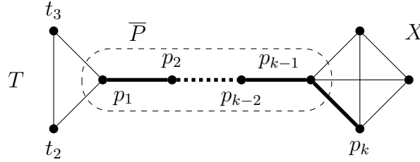
Figure 2: Paths P and \bar{P} connecting dangerous configurations.
