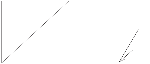
Figure 2: The graph of an 1-comb function and its inverse limit
