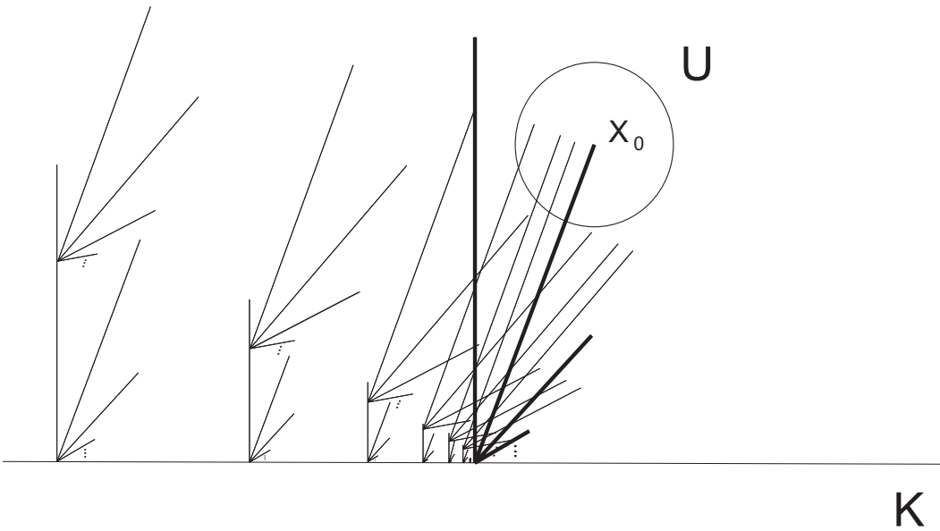
Figure 7: The continuum from Example 3.15
