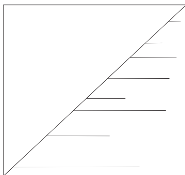
Figure 1: The graph of an 8-comb function
